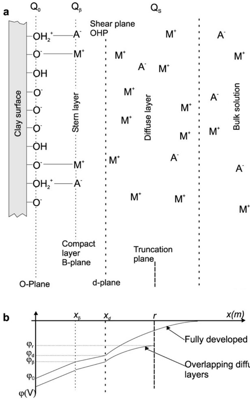
Figure 4: Schematic of the TLM model from ?.
