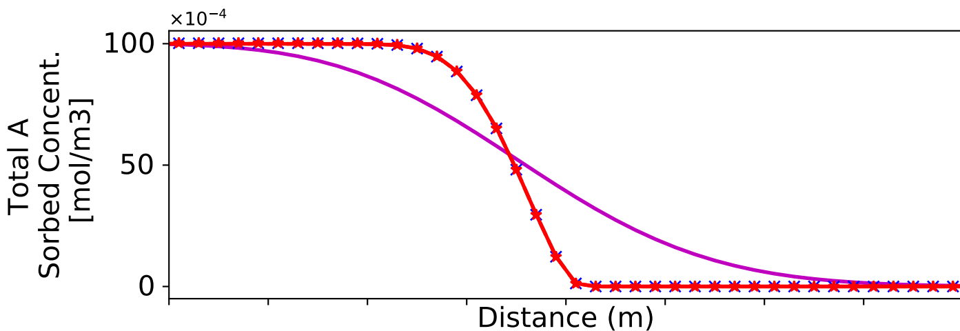
Langmuir and Freundlich sorption models
